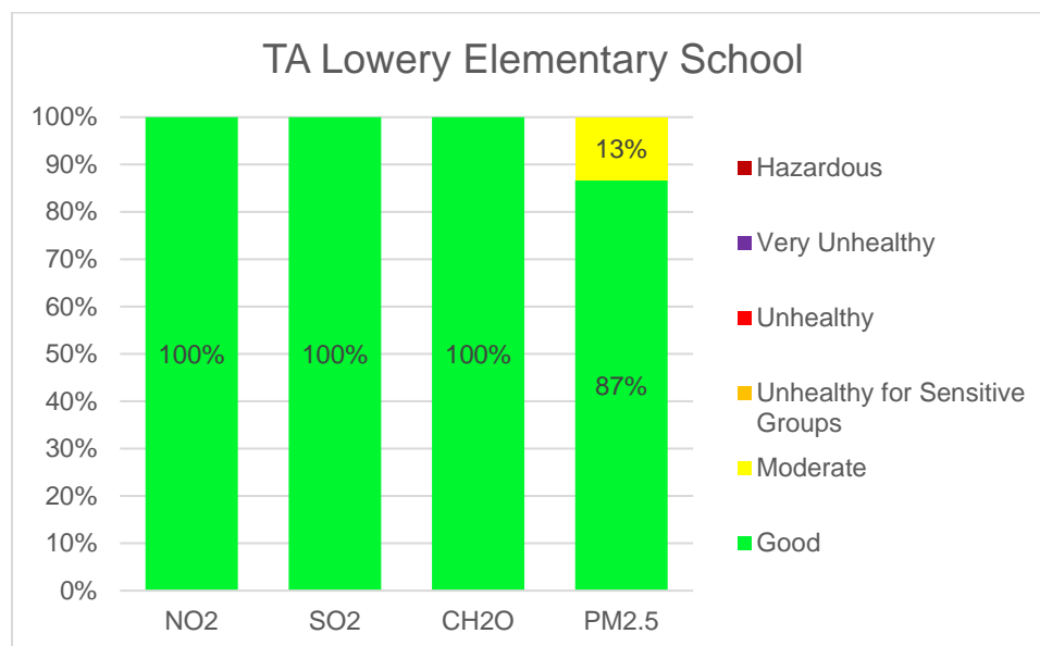
Figure 2: TALES AQI Distribution Summary — January through March 2023
