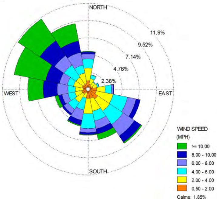
Figure 12: January through March 2023 Wind Rose
