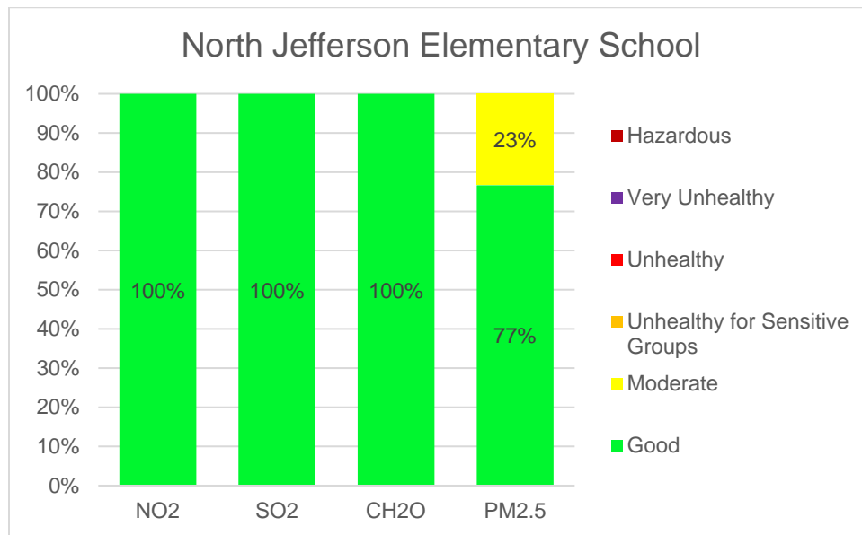
Figure 1: NJES AQI Distribution Summary — January through March 2023
