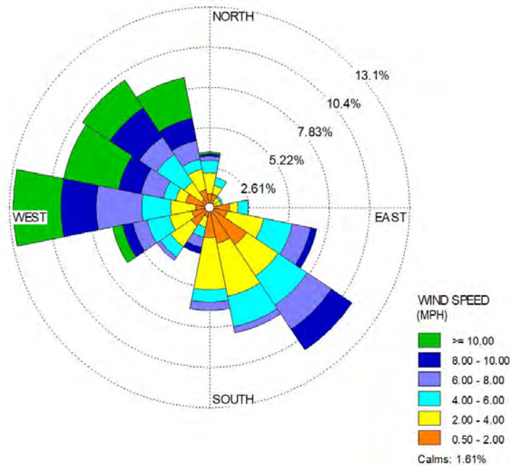
Figure 9: January 2023 Wind Rose
