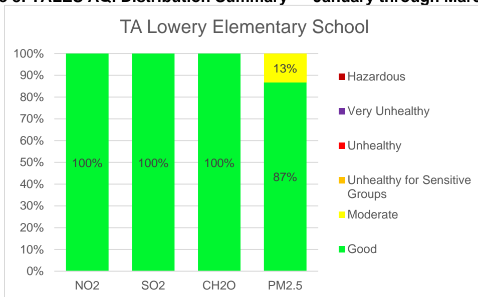
Figure 8: TALES AQI Distribution Summary — January through March 2023
