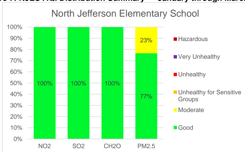
Figure 7: NJES AQI Distribution Summary — January through March 2023
