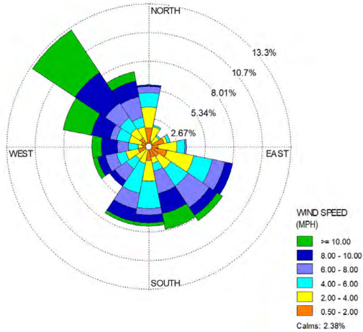
Figure 10: February 2023 Wind Rose
