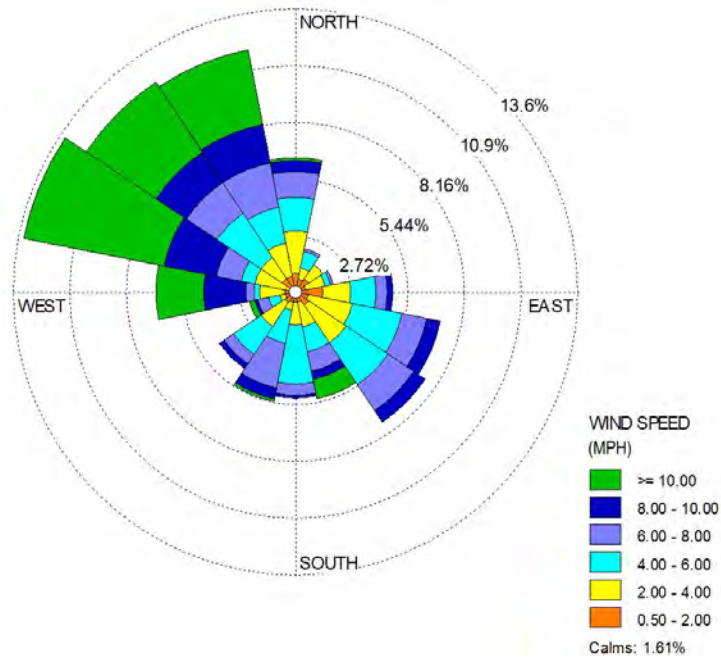
Figure 11: March 2023 Wind Rose
